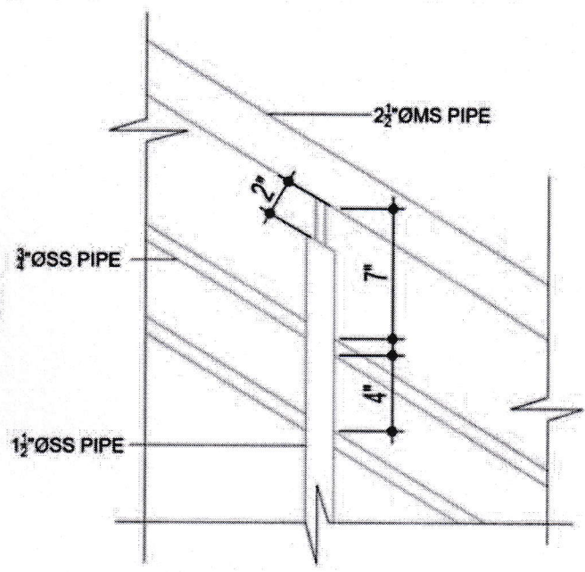
DETAIL SEC.- 7
